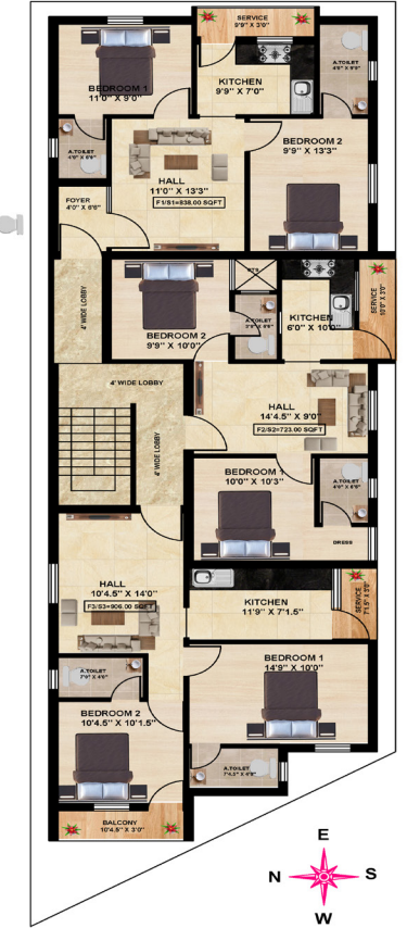
Typical First, Second Floor Plan
